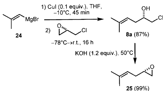
Scheme 7. Synthesis of side-chain precursor 25
