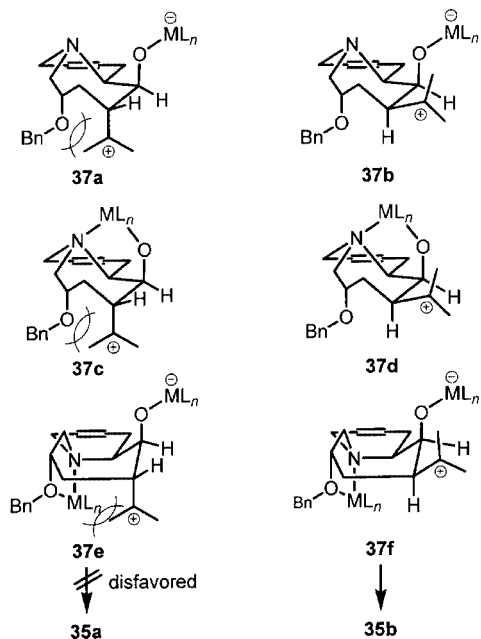
Scheme 12. Assumed transition state geometries 37a–f in the Lewis-acid-catalyzed cyclization of aldehyde 33 to product 35b
