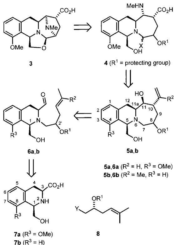
Scheme 2. Retrosynthetic pathway
