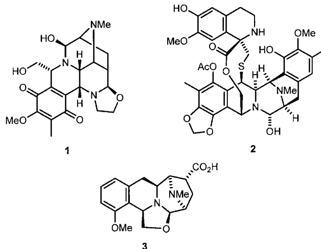
Scheme 1. Tetrahydroisoquinoline alkaloid derivatives 1 – 3
