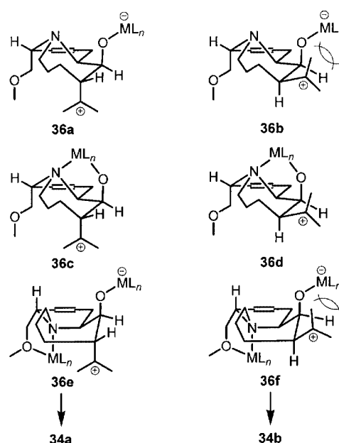
Scheme 11. Assumed transition state geometries 36a–f in the Lewis-acid-catalyzed cyclization of aldehyde 27 to products 34
