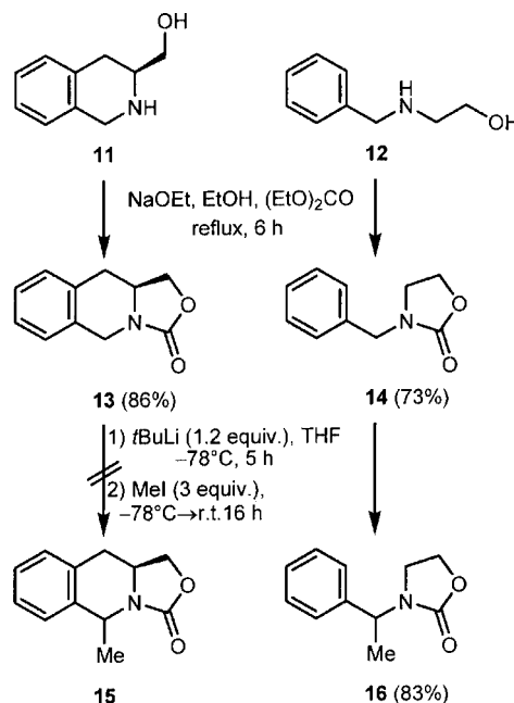
Scheme 4. Alkylation of tricyclic oxazolidinone 13 and structurally related compound 14
