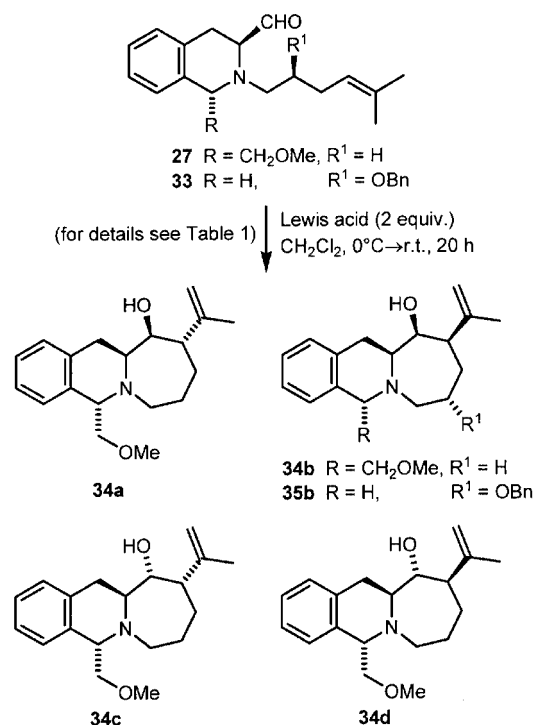
Scheme 10. Lewis-acid-catalyzed cyclization of derivatives 27 and 33 [19d] to diastereomers 34a–d and 35b , respectively; 40 h reaction time in the conversion of 33
