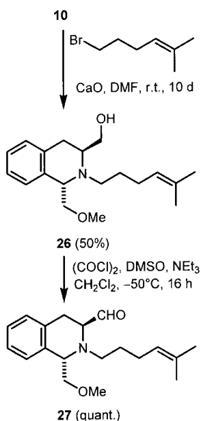
Scheme 8. Synthesis of unfunctionalized cyclization precursor 27
