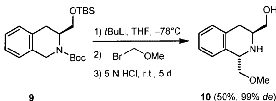
Scheme 3. Preparation of trans -1,3-disubstituted tetrahydroisoquinoline 10 ; for other electrophiles see ref. [8]
