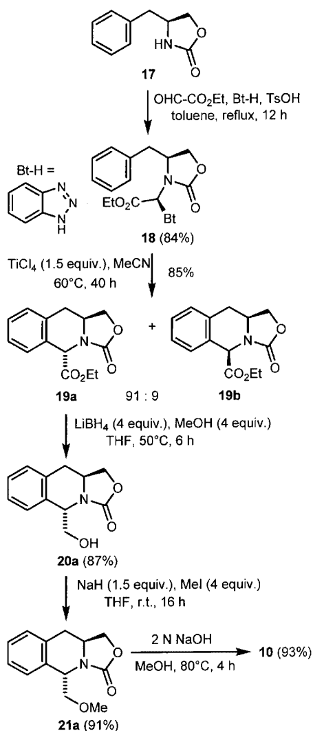
Scheme 5. Synthesis of 1,3-disubstituted tetrahydroisoquinoline 10 by benzotriazole methodology
