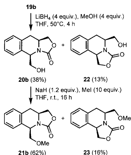
Scheme 6. Conversion of cis -ester 19b
