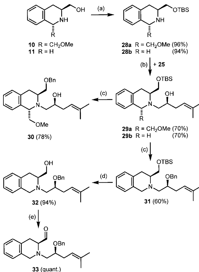
Scheme 9. Introduction of a chiral side chain; reagents and conditions: (a) TBSCl, imidazole, DMAP, \text{CH}_2\text{Cl}_2 , room temp., 16 h; (b) \text{AlEt}_3 (1.3 equiv.), 25 , \text{CH}_2\text{Cl}_2 , room temp., 16 h; (c) 1) \text{NaOtBu} (1.2 equiv.), \text{BnBr} (1.5 equiv.), THF, room temp., 16 h; (d) TBAF (3 equiv.), THF, room temp., 24 h; (e) (\text{COCl})_2 , DMSO, \text{NEt}_3 , \text{CH}_2\text{Cl}_2 , -50^{\circ}\text{C} , 16 h
